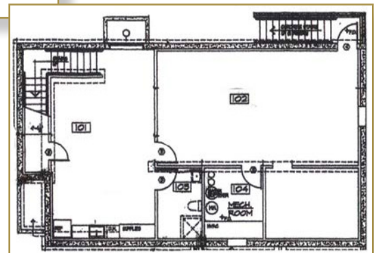
Lower Floor
