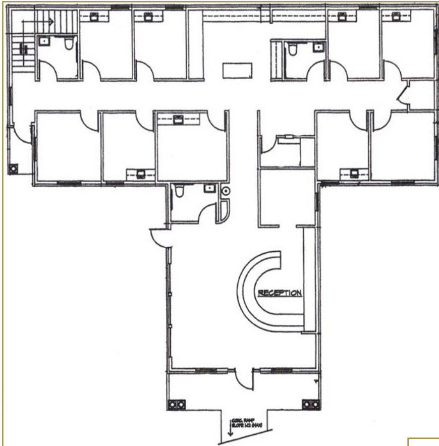
Main Floor
